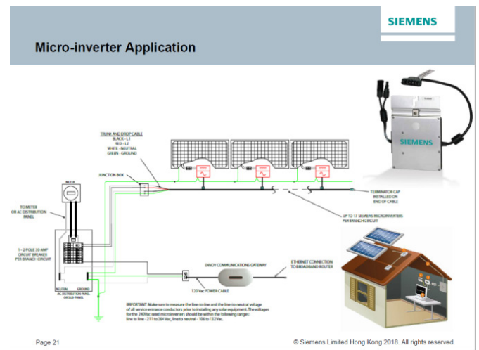
Application of Micro-inverter for power generation
